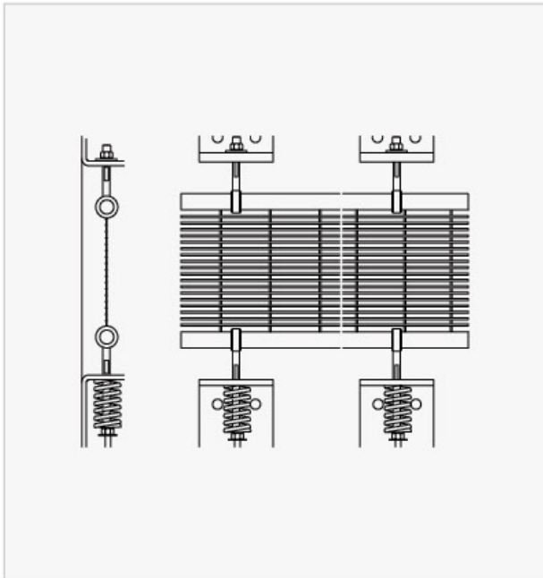
幕墙内外装饰网安装示意图 Installation Diagram Of Curtain Wall Interior And Exterior Decorative Mesh
